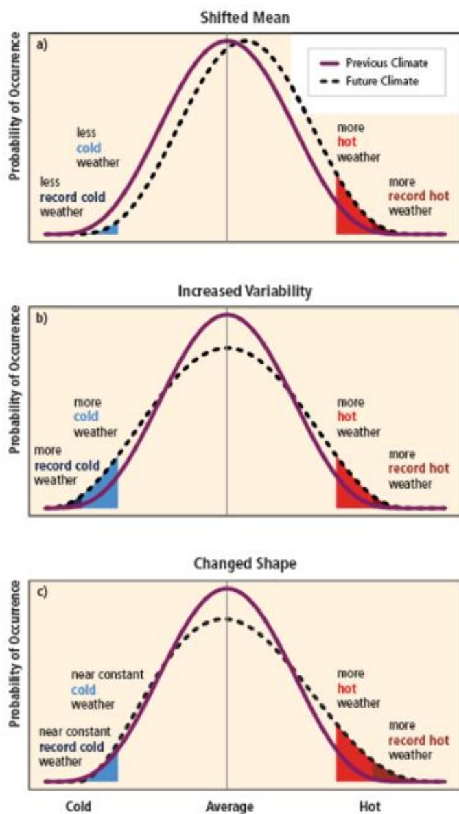
Figure 3: The effect of changes in temperature distribution on extremes.
